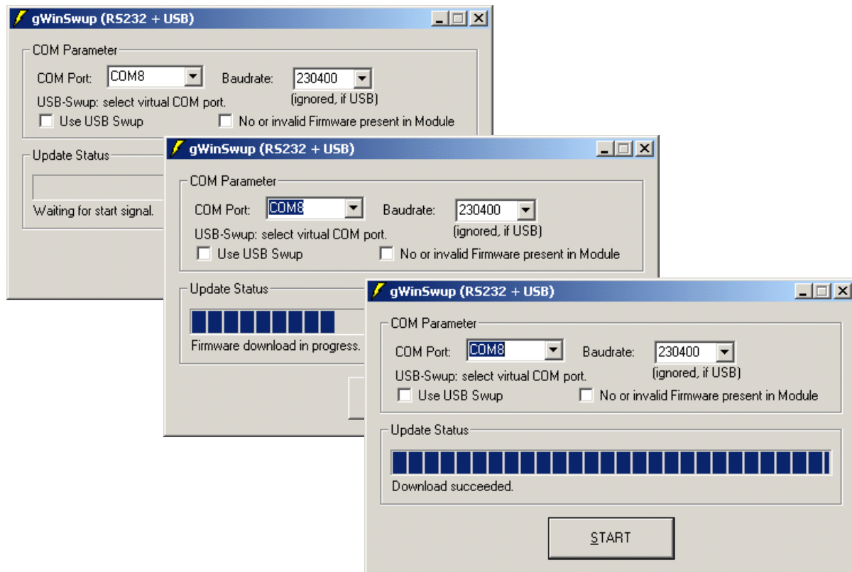
Figure 1: gWinSwub download via ASC0
