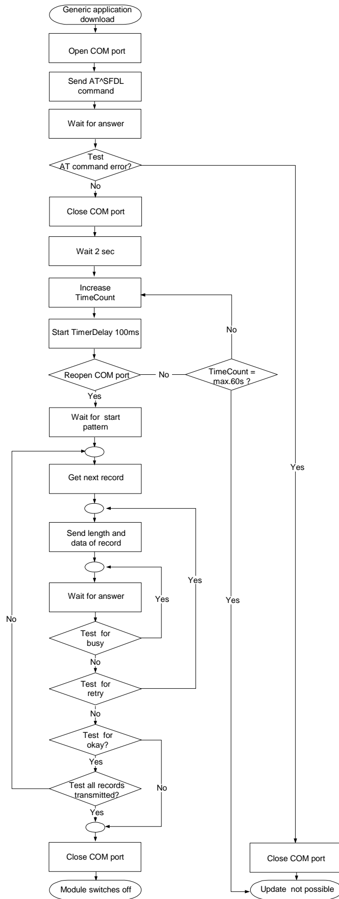
Figure 8: Download protocol for USB
