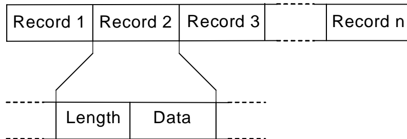
Figure 6: Format of *.USF firmware file
